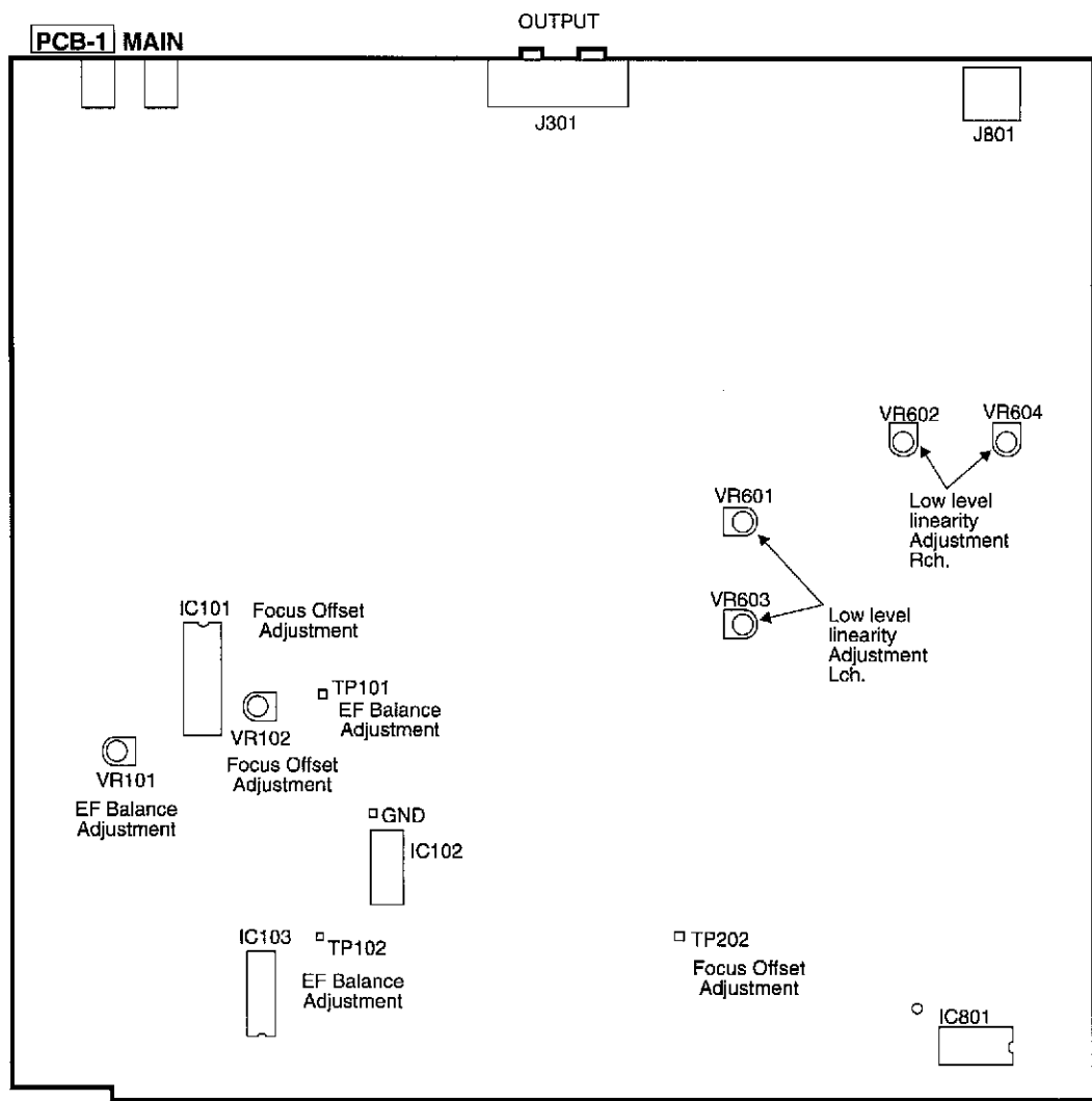
ADJUSTMENT POINT
